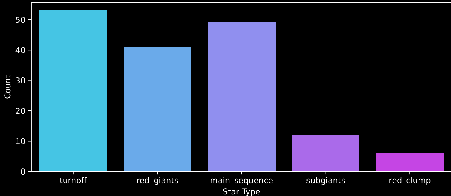
GALAH DR4 Field: [7128] Count plot of Star Type
