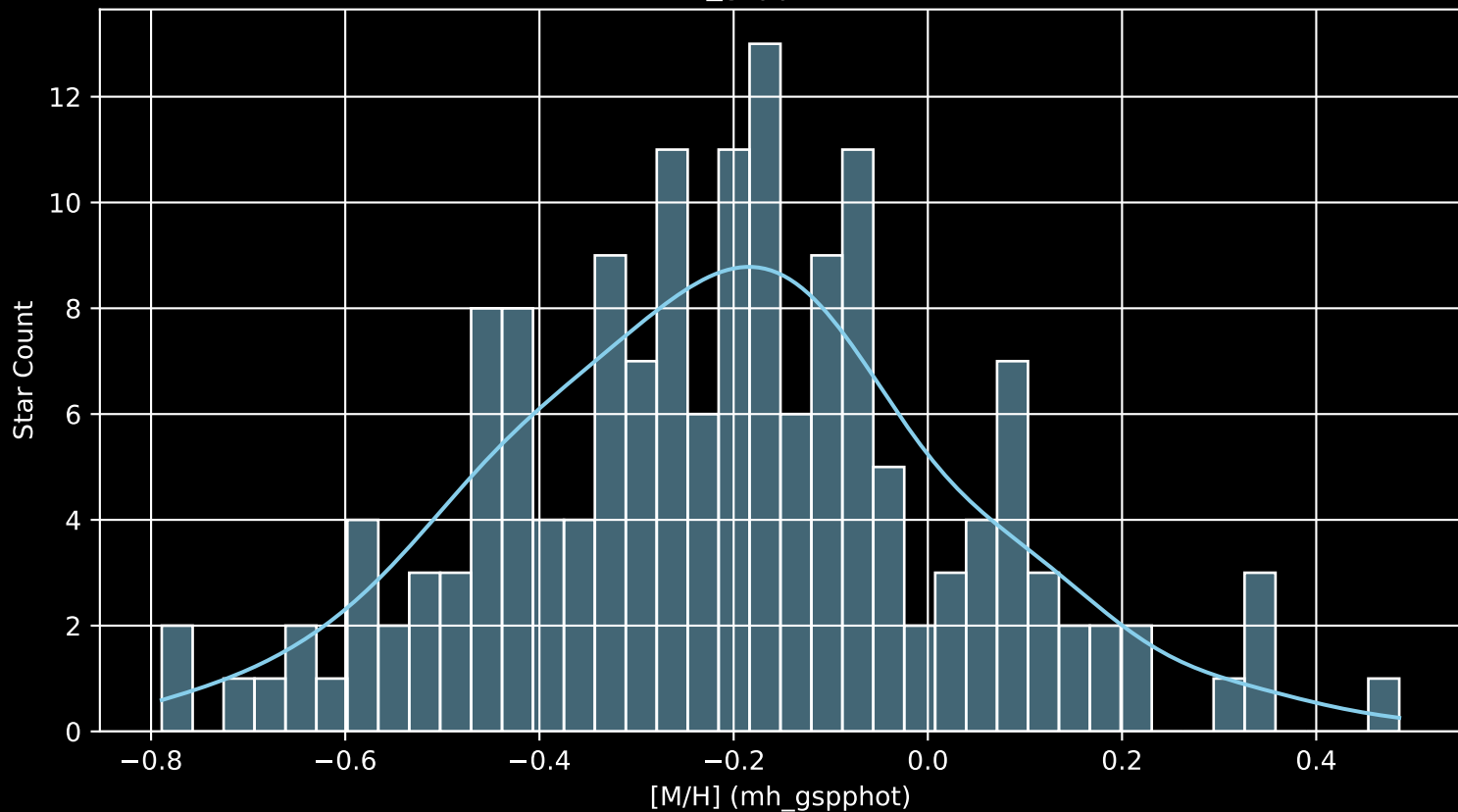
GALAH DR4 Field: [7128] [M/H] (mh_gspphot) (n= 161)
