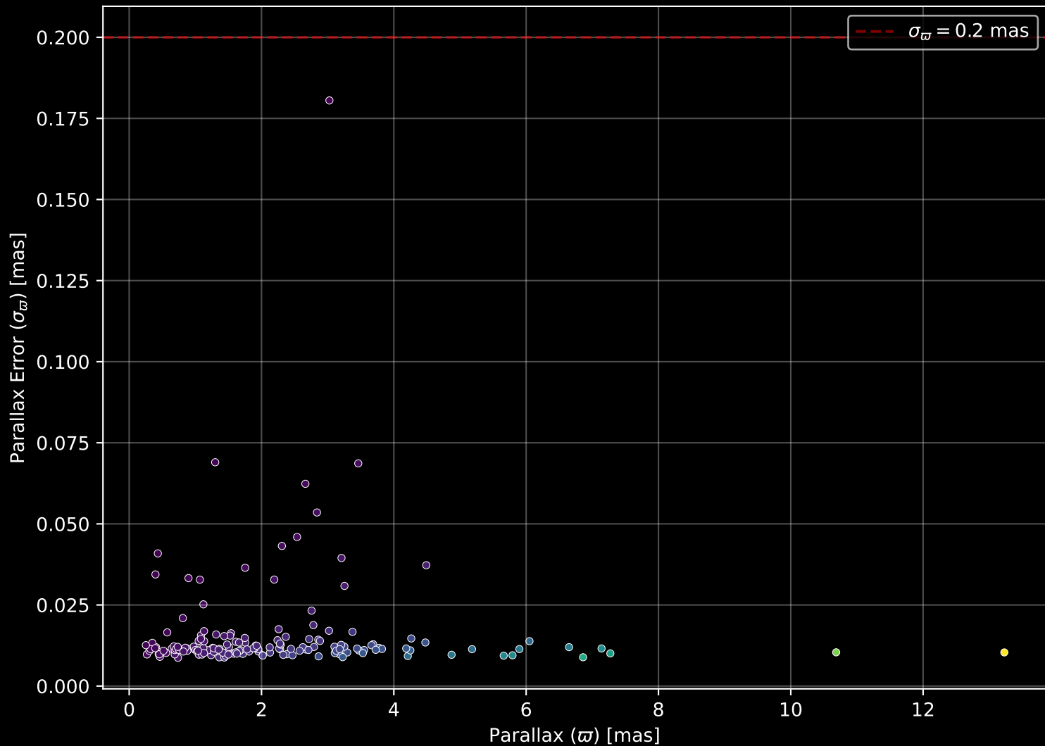
GALAH DR4 Field: [7128] Parallax Quality (n= 161)
