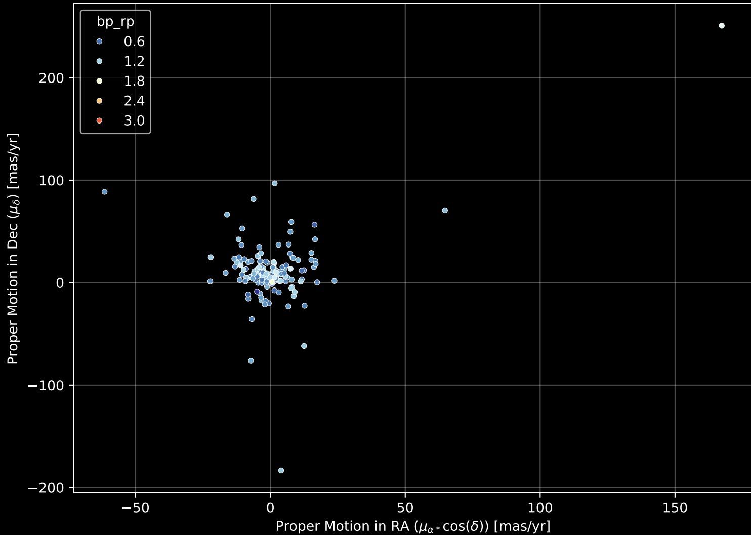
GALAH DR4 Field: [7128] Proper Motion Diagram (n= 161)
