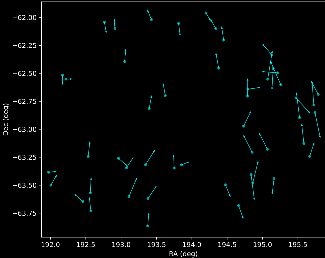
GALAH DR4 Noise Stream Proper Motion Vectors (n=49)
