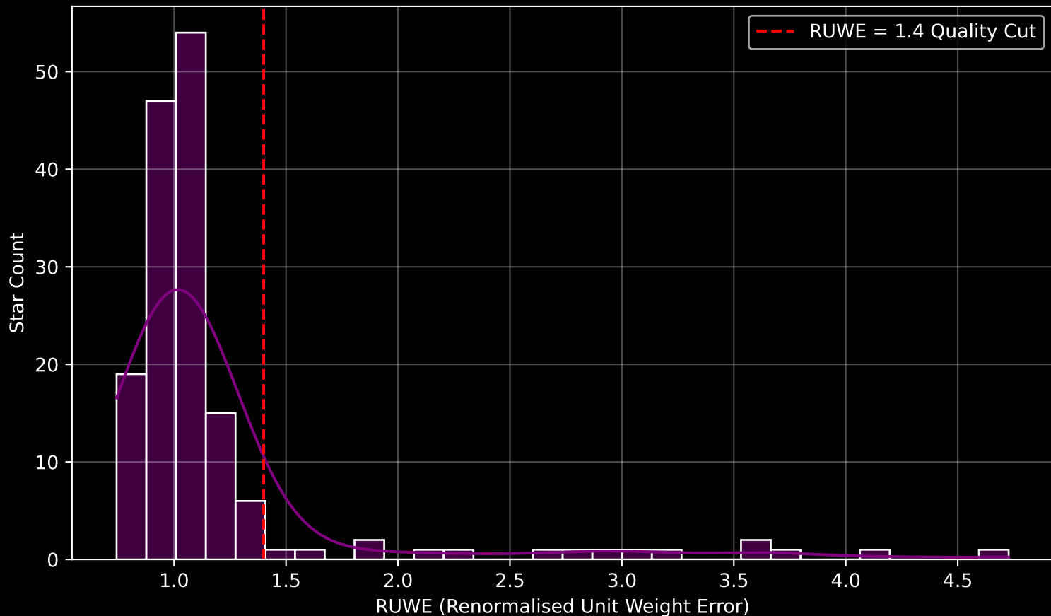
GALAH DR4 Field [7128] RUWE Distribution (n= 157)
