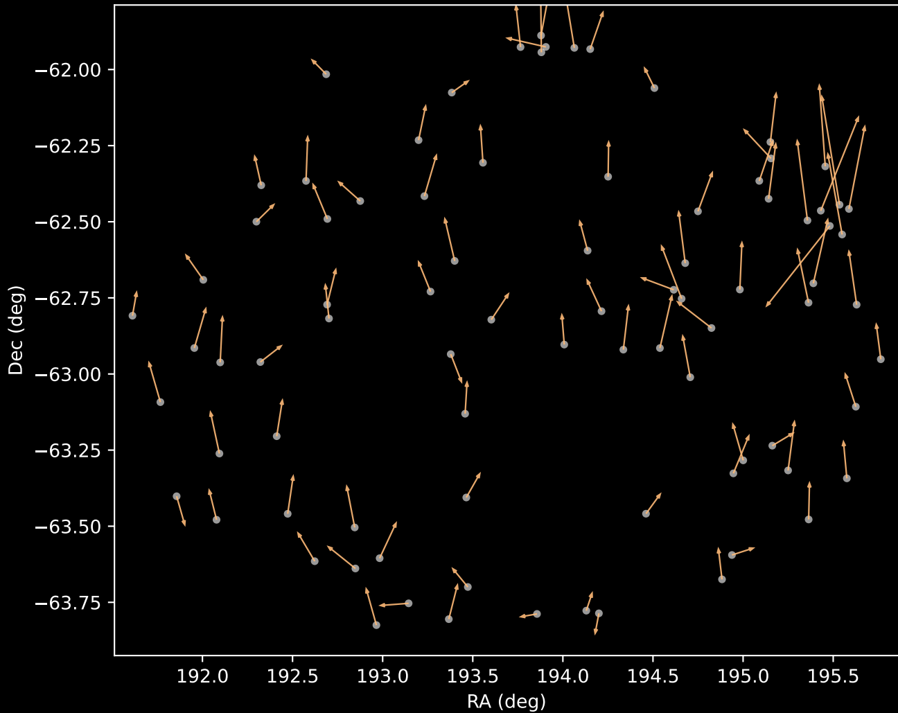
GALAH DR4 Cluster 3 Proper Motion Vectors (n=85)
