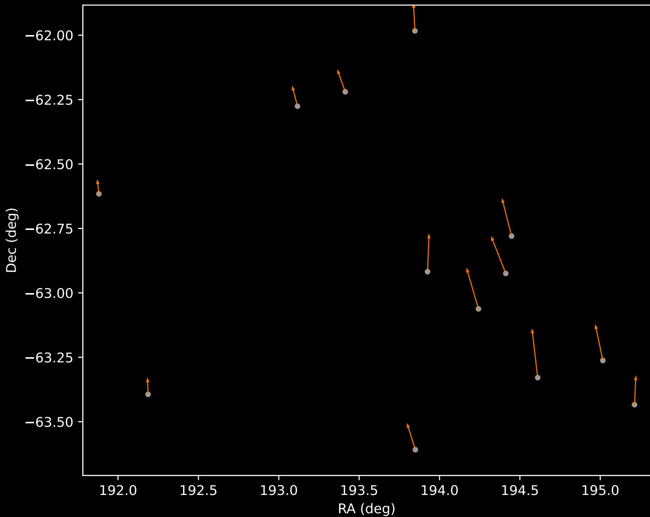
GALAH DR4 Cluster 2 Proper Motion Vectors (n=13)
